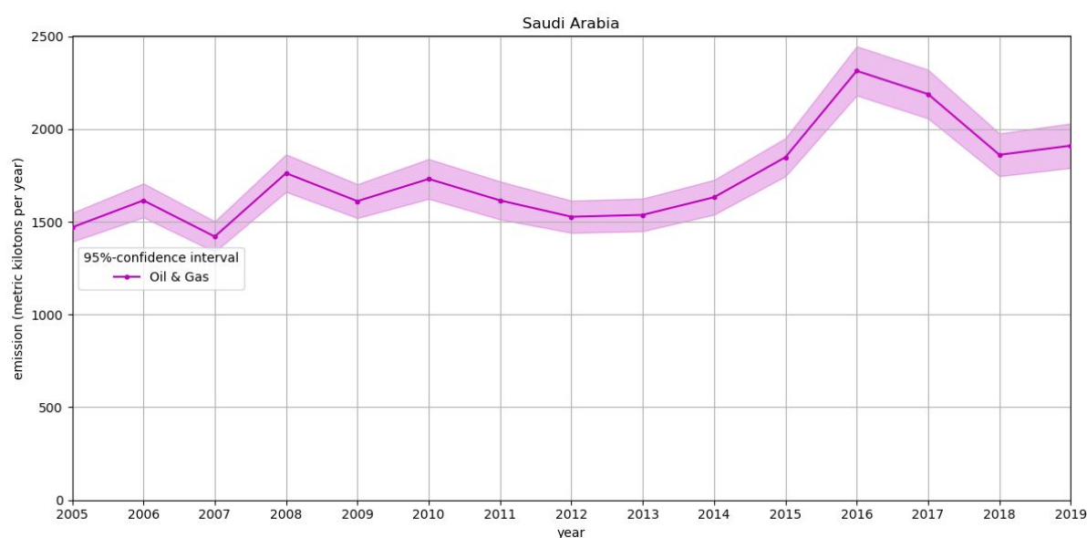
Figure 10: Contributions of major industry sectors to total \text{SO}_2 emissions from 2005 to 2019 in Saudi Arabia (kilotonnes per year). Data source: NASA MEaSUREs.
