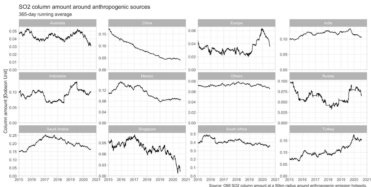
Figure 23: The 2015–2020 SO 2 column amounts within 50km of anthropogenic sources in countries that have large emissions. 365-day running average. ‘Others’ refers to all other countries combined. Data source: OMI.
